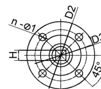
Mounting flange ISO 5211
